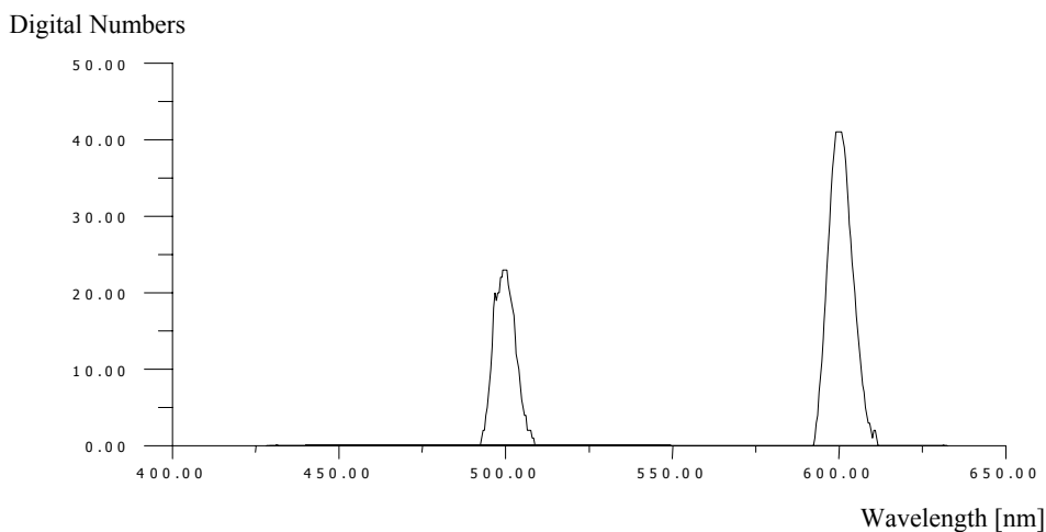
Fig.4. Spectral response functions for channel 500nm and channel 600nm.
