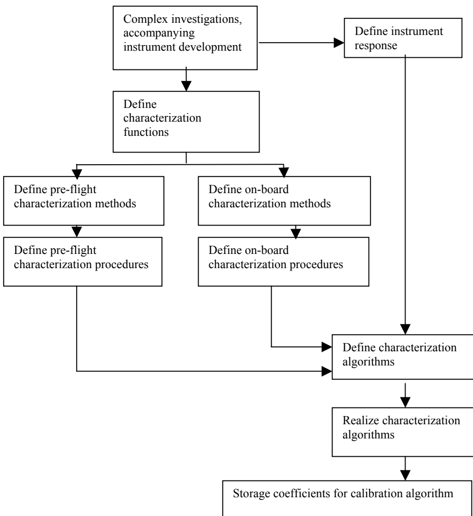
Fig. 1. Preprocessing steps for imaging spectrometer data
